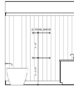
3 PRIMARY BATH - ELEVATION 2 1/2" = 1'-0"
