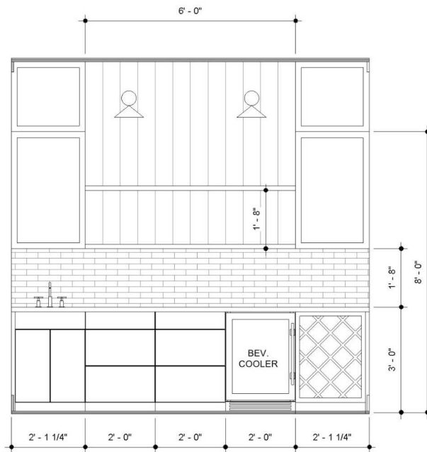
7 WET BAR - ELEVATION 1 1/2" = 1'-0"
