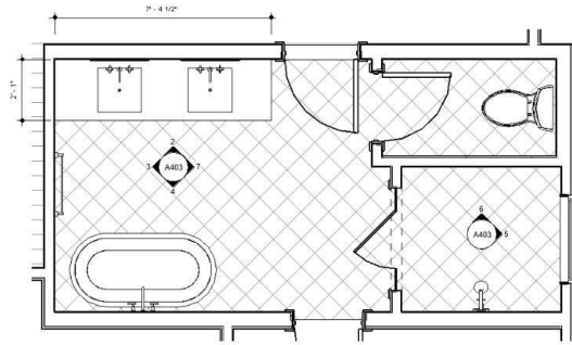
1 PRIMARY BATH - ENLARGED PLAN 1/2" = 1'-0"
