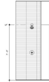
3 BATH 113 - ELEVATION 2 1/2" = 1'-0"
