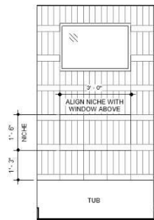
3 BATH 203 - ELEVATION 2 1/2" = 1'-0"
