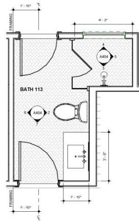
1 BATH 113 - ENLARGED PLAN 1/2" = 1'-0"
