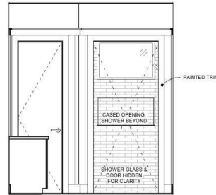
7 PRIMARY BATH - ELEVATION 4 1/2" = 1'-0"
