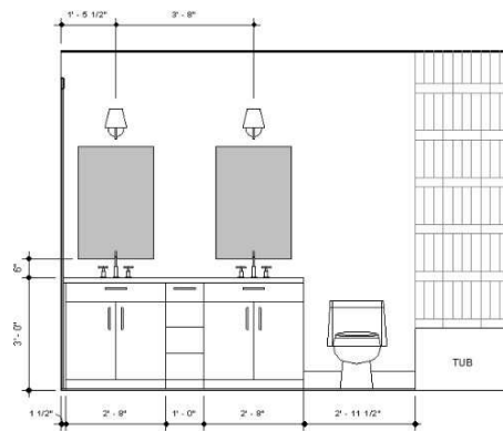
2 BATH 203 - ELEVATION 1 1/2" = 1'-0"
