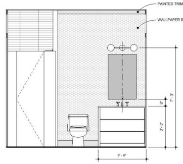
2 BATH 113 - ELEVATION 1 1/2" = 1'-0"
