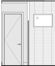
4 BATH 113 - ELEVATION 4 1/2" = 1'-0"
