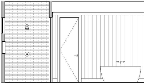
4 PRIMARY BATH - ELEVATION 3 1/2" = 1'-0"
