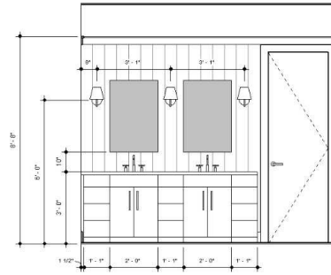
2 PRIMARY BATH - ELEVATION 1 1/2" = 1'-0"
