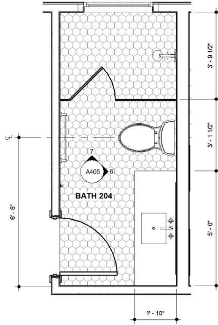
5 BATH 204 - ENLARGED PLAN 1/2" = 1'-0"
