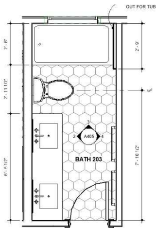
1 BATH 203 - ENLARGED PLAN 1/2" = 1'-0"
