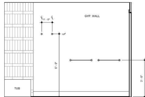
4 BATH 203 - ELEVATION 3 1/2" = 1'-0"
